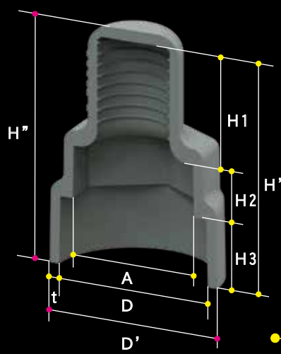
断面図 [Cross section]
