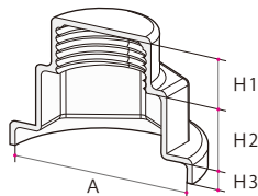
断面図 [Cross section]
