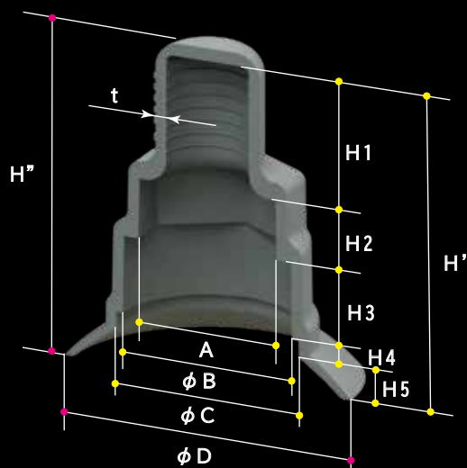
断面図 [Cross section]
